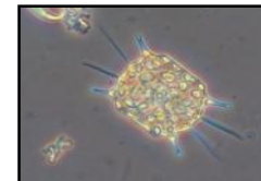
Odontella
