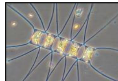
Chaetoceros
